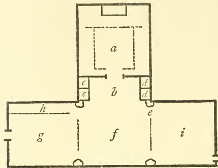
The Ichnography 1 of Merton College Church.
